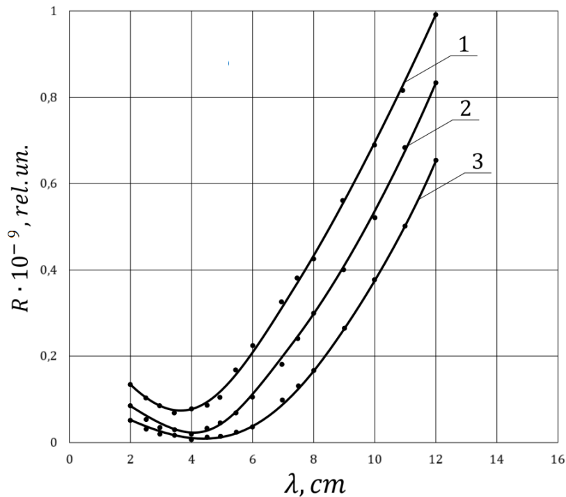
Figure 4. The dependence of the reflection coefficient R from wavelength \lambda . Graphs 1, 2 и 3 correspond to the values of ^{16}\text{N} isotope ions concentration N_i in \text{cm}^{-3} : 10^{10} ; 10^9 ; 10^8 .
