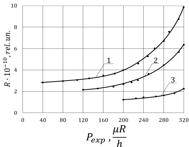
Figure 3. The dependence of the reflection coefficient R from the power of the exposure dose P_{\text{exp}} for different wavelengths \lambda of microwave radiation. Graphs 1, 2 and 3 correspond to the values of the radiation wavelength \lambda in cm: 8; 5; 2.
