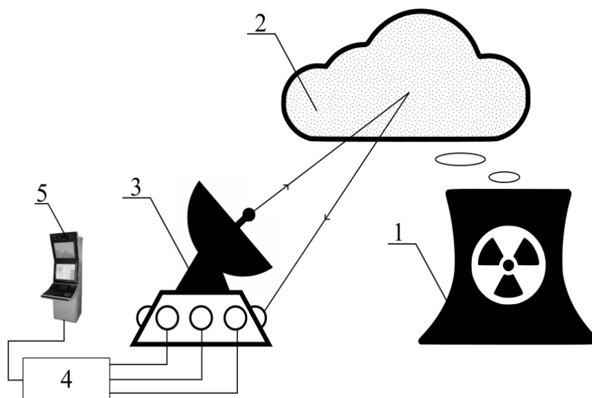
Figure 1. Block diagram of the radar for detecting and investigating radioactive contamination in the atmosphere: 1 – a source of radioactive emissions; 2 – a cloud of ionized particles (plasmoid); 3 – an antenna complex developed by us; 4 – a receiving path with a FOCL developed by us; 5 – device for detecting and processing signals (control case).
