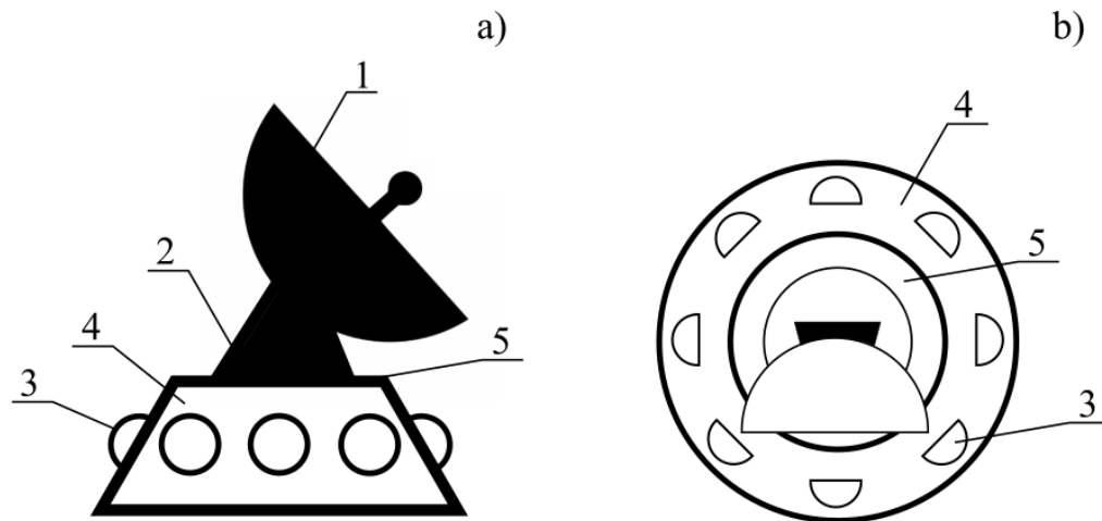
Figure 2. Structural diagram of the radar antenna complex (a – side view, b – top view): 1 – parabolic antenna; 2 – system for scanning the parabolic antenna in the vertical plane, 3 – spiral receiving antennas; 4 – fixed support for mounting spiral antennas; 5 – movable part of the support for rotating the parabolic antenna 360 degrees
